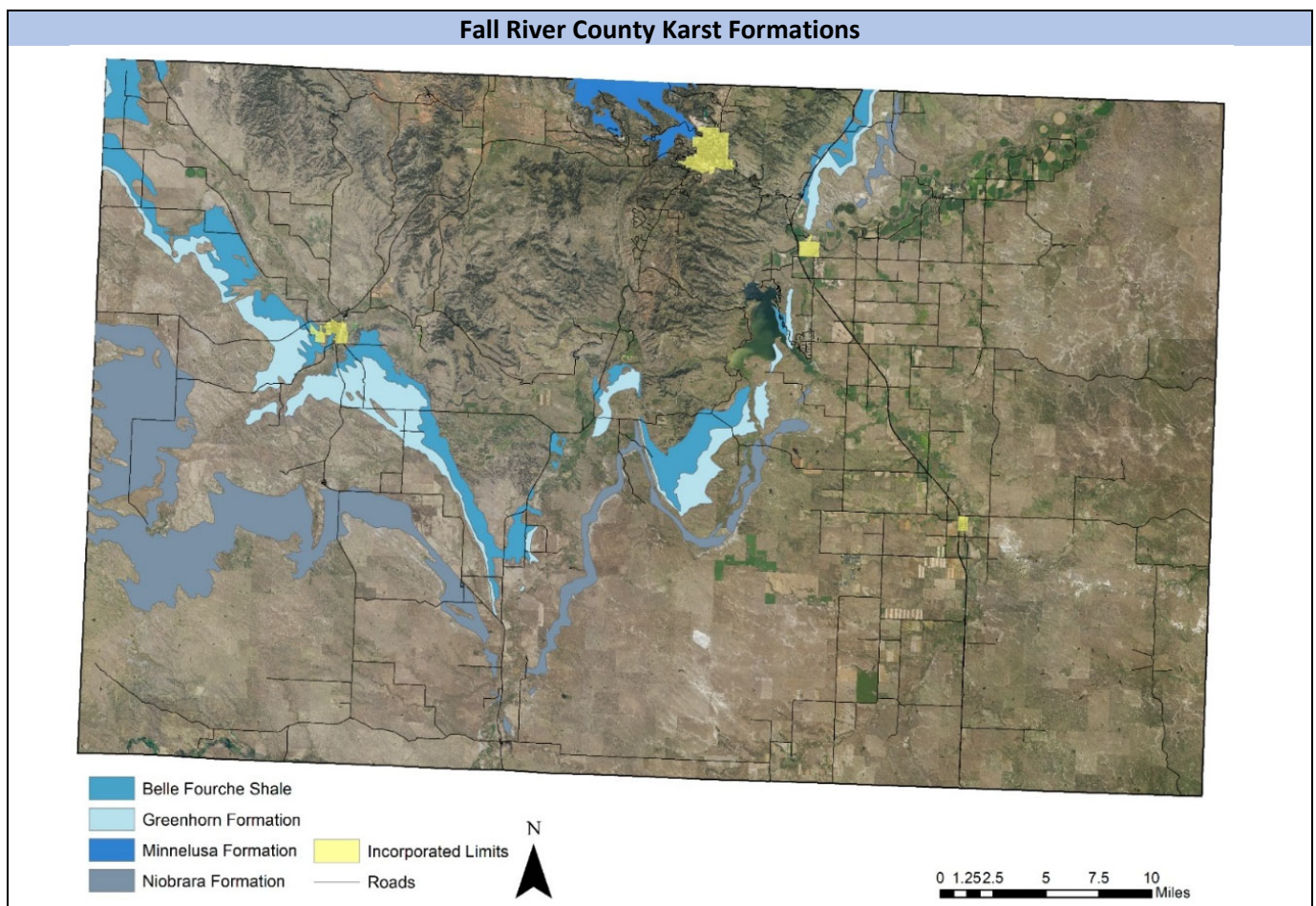
Figure 3.16. Fall River County Karst Formations. Source: USGS. (Requirement B1-b)
